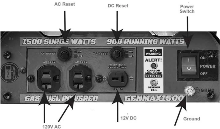
Figure 8 - Outlets available on this generator
