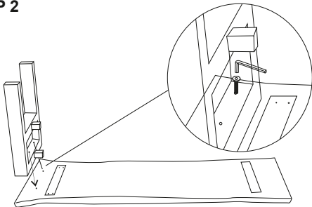
LEG (2 PIECES)
