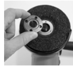
Figure 3 Grinder with spindle facing up
