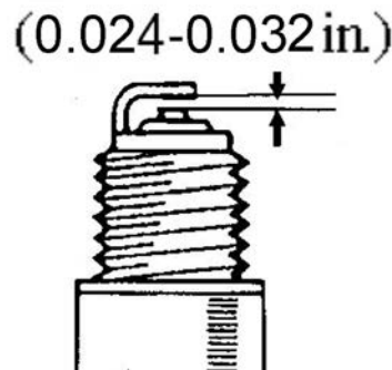
Figure 9 Measuring the spark plug gap
